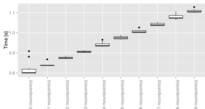
Figure 2. Access time with 1000 keys with 100000 iterations and an increasing number of mountpoints. Note that the high number of iterations means that the relative time is very low.
