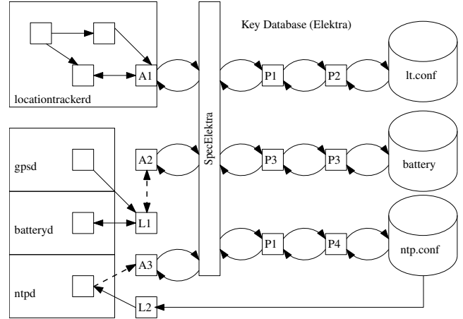
Figure 1. Horizontal and vertical modularity of locationtracker device. Boxes are applications, cylinders are configuration files, A? are adapter libraries, L? are configuration libraries, P? are plugins.
